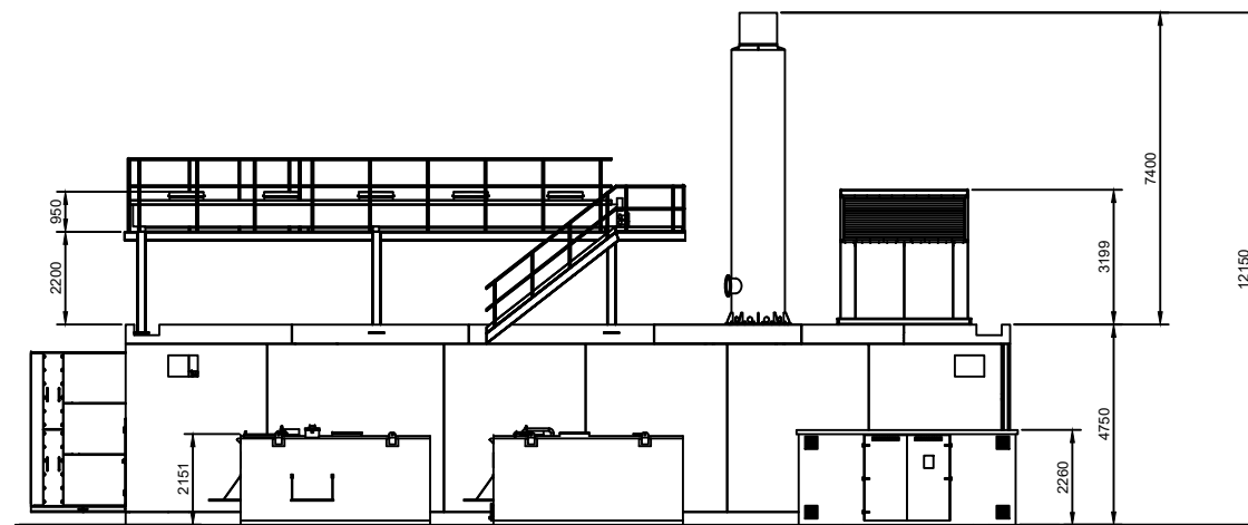
EASTERN ELEVATION
